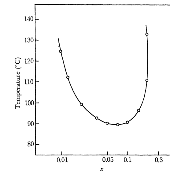
Fig. 1. The liquid-liquid phase diagram for the TGDE+water system.
